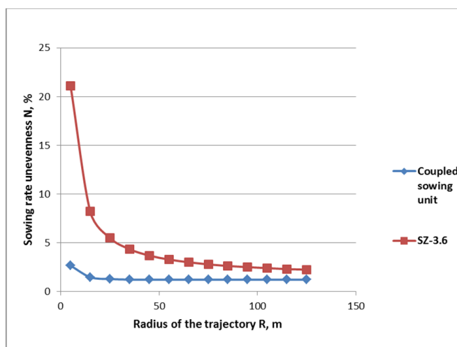
Figure 1 Relationship between seeding rate unevenness N and the trajectory radius R
